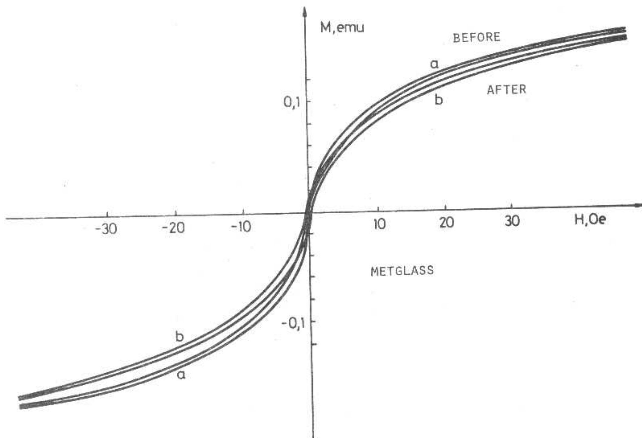
Fig. 16. Magnetization curve of metglass sample \text{Fe}_{75}\text{Cr}_5\text{B}_{20} before (curve a) and after (curve b) activation.
