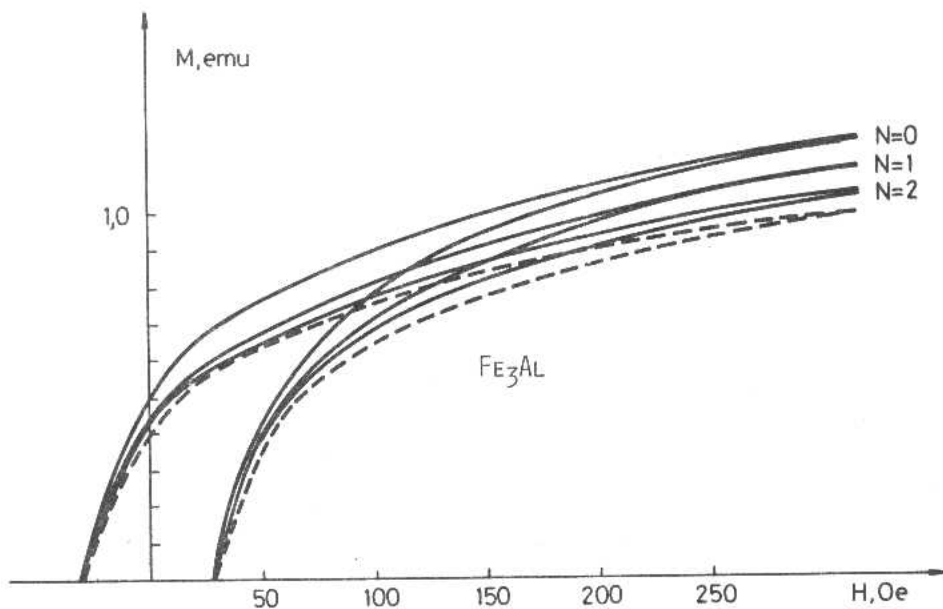
Fig. 11. Magnetization curve of \text{Fe}_3\text{Al} sample before (broken curve) and after (solid curves) activation. Parameter N represents the number of days after activation.
