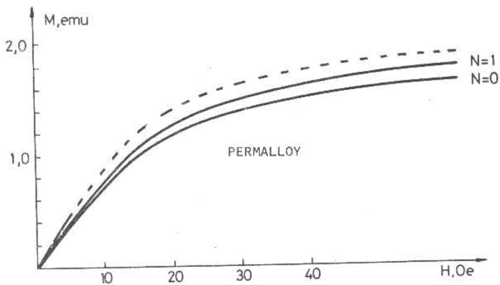
Fig. 12. Change of the magnetization curve of the permalloy sample of Fig. 9 in time. (Broken curve: before activation, solid curves: after activation, N : number of days after activation).
